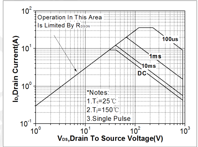
Fig. 10. Maximum safe operating area(TO-3P)
