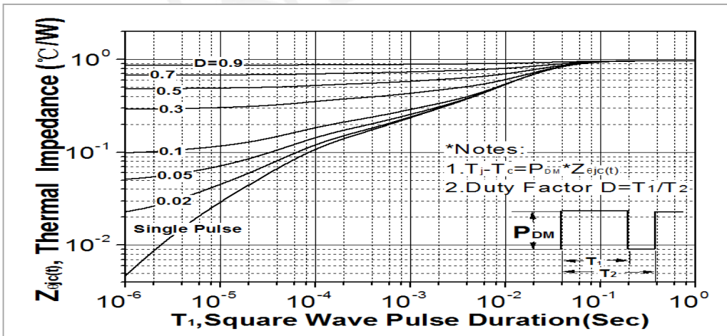
Fig. 11. Transient thermal response curve (TO-252&TO-251)
