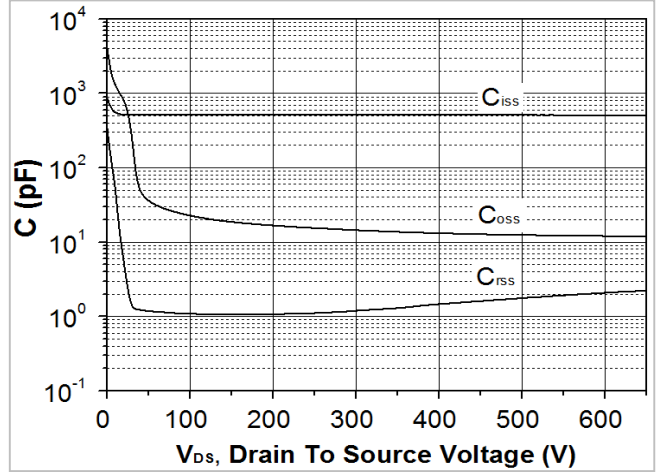
Fig. 8. Capacitance Characteristics
