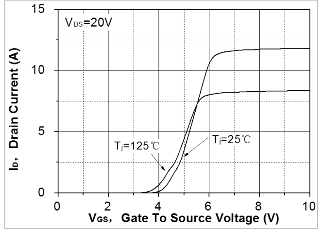
Fig. 2. Transfer Characteristics
