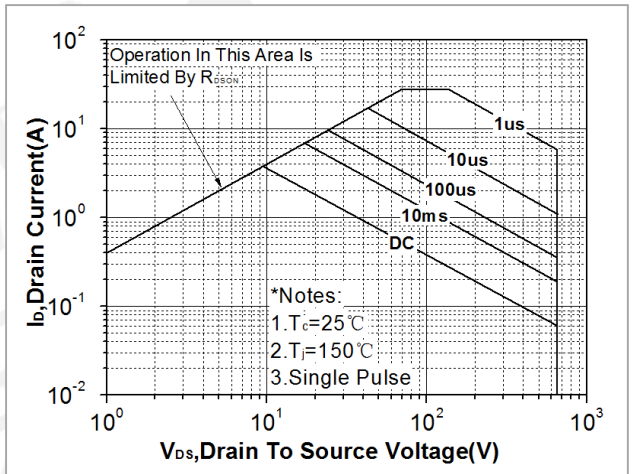
Fig. 10. Maximum safe operating area (TO-220F&TO-220FTN)
