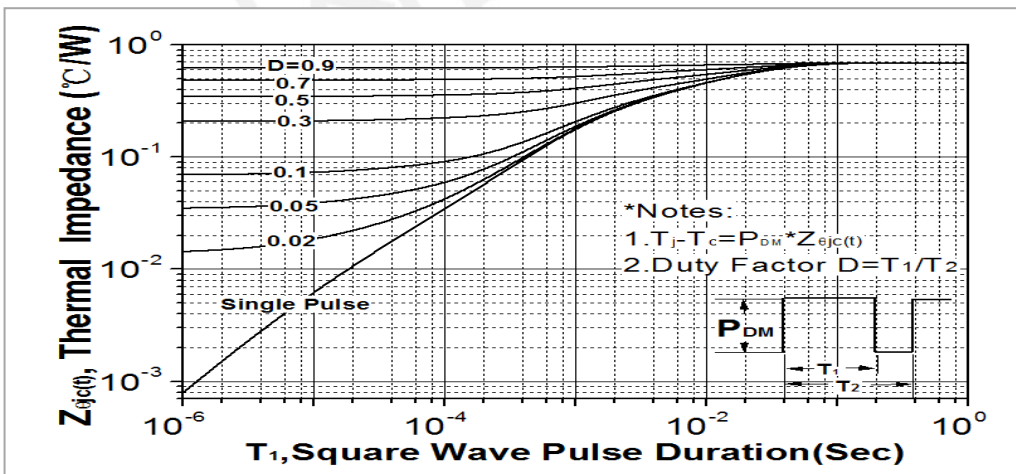
Fig. 11. Transient thermal response curve(TO-262N)
