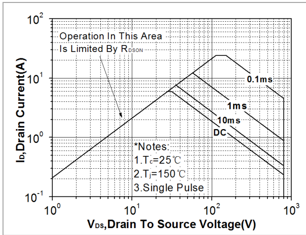
Fig. 9. Maximum safe operating area(TO-262N)
