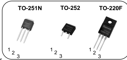
1. Gate 2. Drain 3. Source
