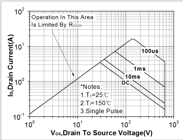
Fig. 9. Maximum safe operating area (TO-252 & TO-251N)
