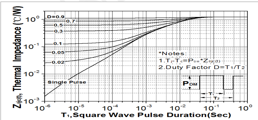
Fig. 10. Transient thermal response curve (TO-252 & TO-251N)
