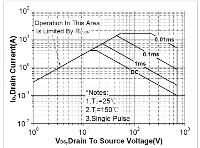
Fig. 8. Maximum safe operating area (TO-251N&TO-251N)
