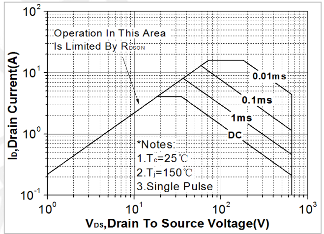
Fig. 10. Maximum safe operating area (TO-251N/TO-252/TO-251S)
