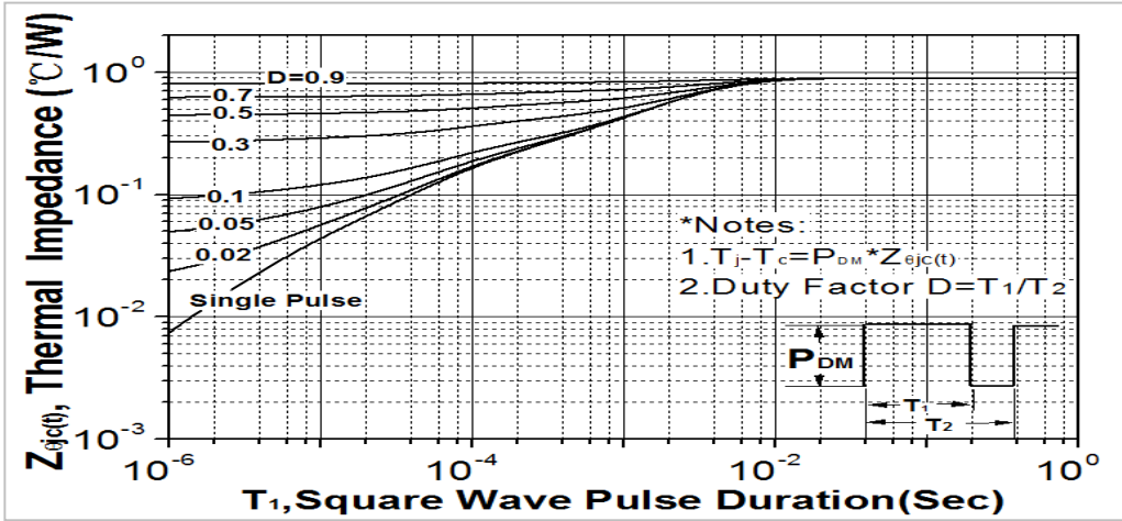
Fig. 12. Transient thermal response curve(TO-251N/TO-252/TO-251S)
