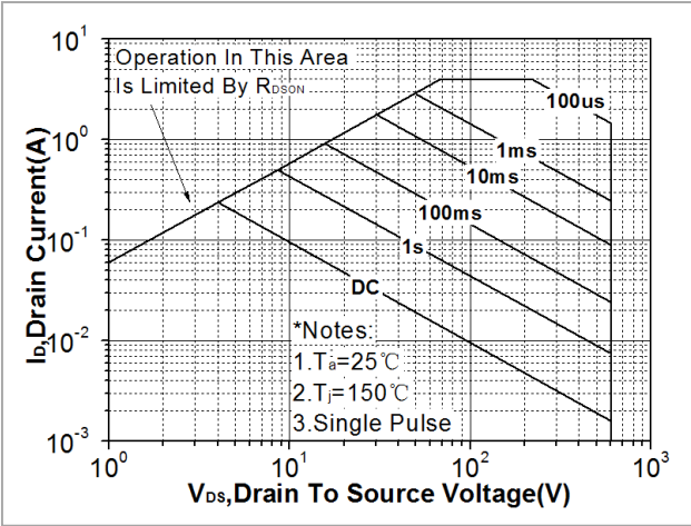
Fig. 9. Maximum safe operating area(TO-92)
