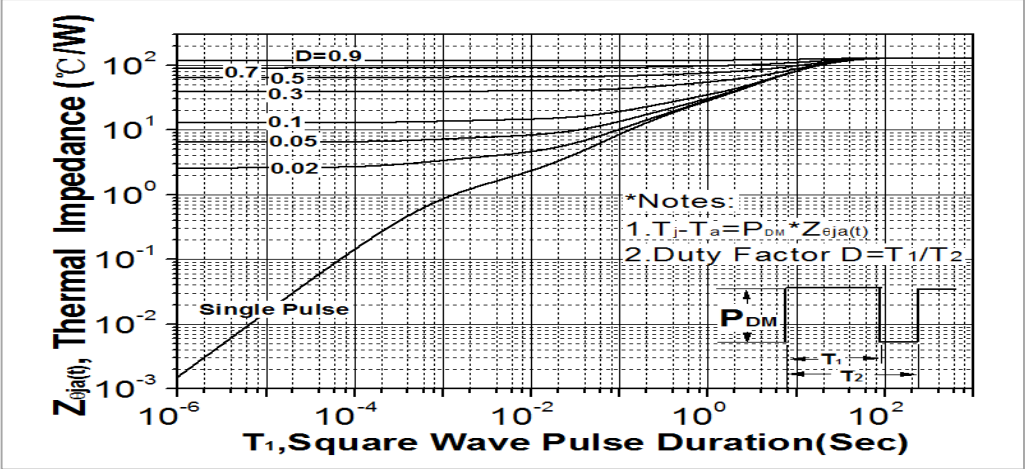
Fig. 11. Transient thermal response curve(TO-92)
