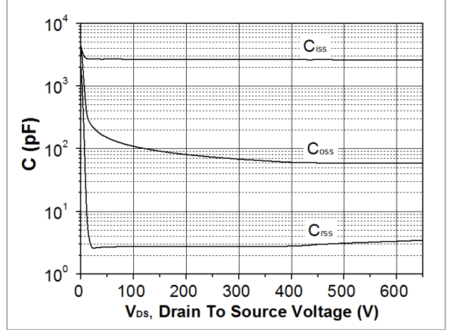
Fig. 8. Capacitance Characteristics
