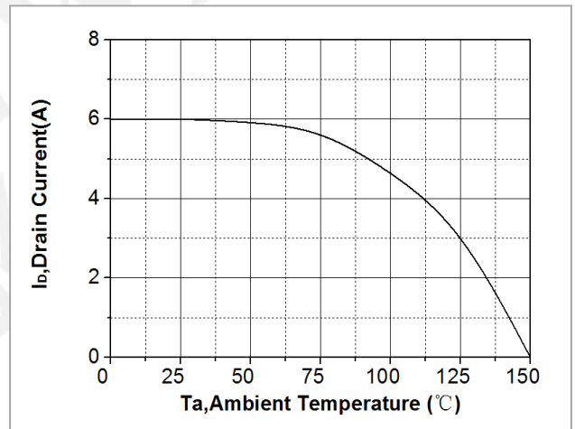
Fig. 10. Maximum drain current vs. ambient temperature
