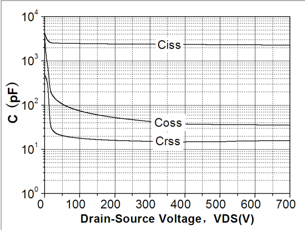
Fig. 11. Capacitance Characteristics
