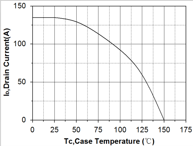
Fig. 10. Maximum drain current vs. case temperature (TO-22FB0&TO-263)
