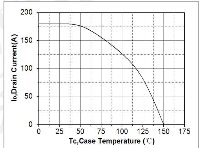
Fig. 10. Maximum drain current vs. case temperature (TO-263&TO-220)
