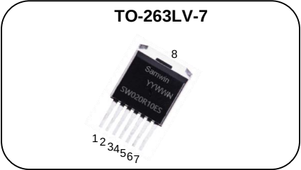
1. Gate 8.Drain 2~7.Source
